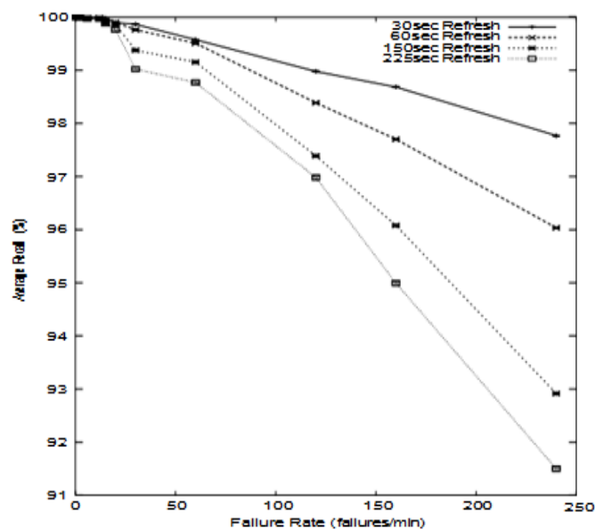
Figure.6 Average recall for different refresh periods.
