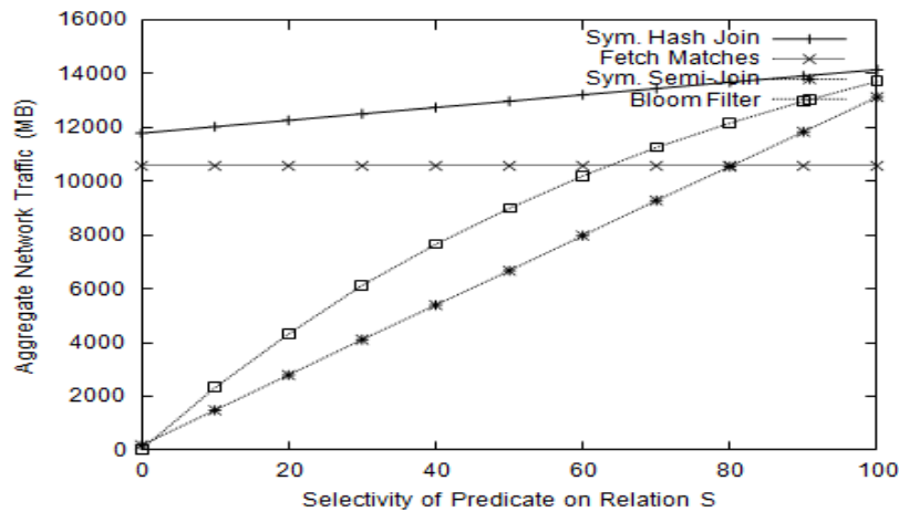
Figure.4 Aggregate network traffic generated by each join strategy.
